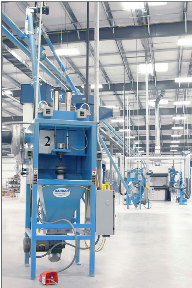
Custom knock-out station with attached Helix® flexible screw conveyor that moves the lightweight, chunky plaster to the sealed tubular drag conveyor for removal to an outside receptacle.
